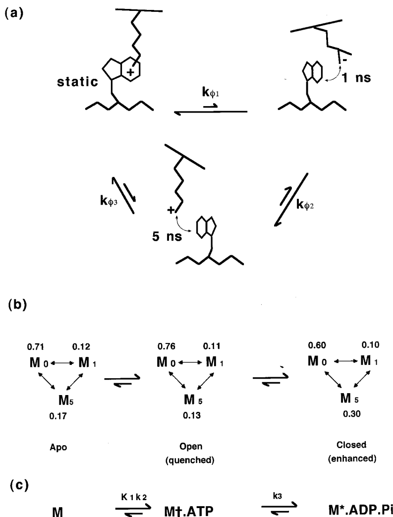
FIG. 4. Schematic diagram to show the interconversion of Trp-501 microstates and their relationship to nucleotide states. Panel a, the mechanism of Trp-501 fluorescence quenching involves three microstates, one of which ( M_0 ) is statically quenched (effective fluorescence lifetime = 0), whereas the other two ( M_1 and M_5 ) have lifetimes of close to 1 or 5 ns. Lifetimes are reduced over the natural lifetime of tryptophan by collisional processes that may involve dynamic interactions with charged or polar side chains, backbone carbonyl groups, or solvent water. The interactions shown are chosen arbitrarily for illustration, but potential candidates can be identified (see “Discussion”). Interconversion between microstates must be slower than 5 ns and could involve different rotamers of Trp-501 as illustrated. This would be in accord with the long rotational correlation times reported in Table I, i.e. k\phi values < 20 \mu\text{s}^{-1} . Panel b, microstates are in rapid equilibrium compared with chemical steps and gross conformational changes (i.e. k\phi values > 50 \text{ ms}^{-1} from temperature jump measurements) and are distributed according to the fractional occupancy shown in Table II. Accordingly a unique pathway of interconversion between microstates cannot be defined during transitions between chemical or gross conformational states because they remain close to equilibrium throughout. Note that the decrease in the 5-ns component largely accounts for the observed percentage quench in Trp-501 emission intensity on binding ADP (to give the open state), whereas the increase in the 5-ns component accounts for the percentage enhancement on forming the closed state (hydrolysis to M^* \cdot \text{ADP} \cdot \text{P}_i ). Panel c, corresponding transitions as applied to the first three chemical steps of the ATPase pathway. Rate constants estimated by transient kinetic methods are macroscopic rate constants for the overall population of microstates. It is assumed in the scheme shown that ATP quenches to the same degree as ADP; this has not been proven (12). From stopped-flow measurements it is likely k_2 is > 200 \text{ s}^{-1} , and k_3 = 30 \text{ s}^{-1} (12). However, perturbation methods indicate that the open \rightarrow closed transition may occur as fast as 1,000 \text{ s}^{-1} but requires hydrolysis to drive the equilibrium toward the closed state (A. Málnási-Csizmadia and C. R. Bagshaw, unpublished observations).
